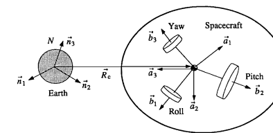
Fig. 6.10 Gyrostatt in a circular orbit.
