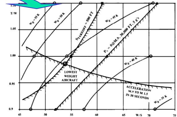
Fig. 19.4 Sizing matrix plot (concluded).
