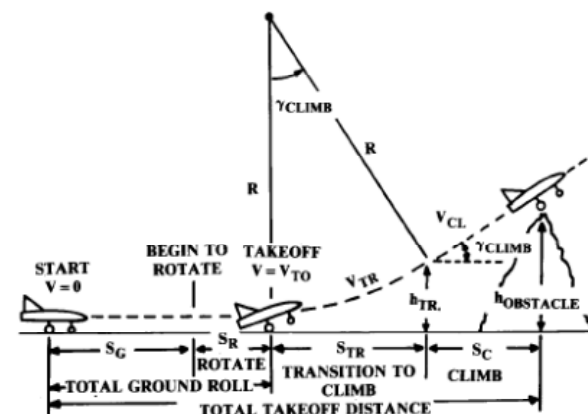
Fig. 17.17 Takeoff analysis.
