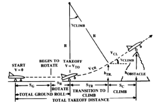
Fig. 17.17 Takeoff analysis.
