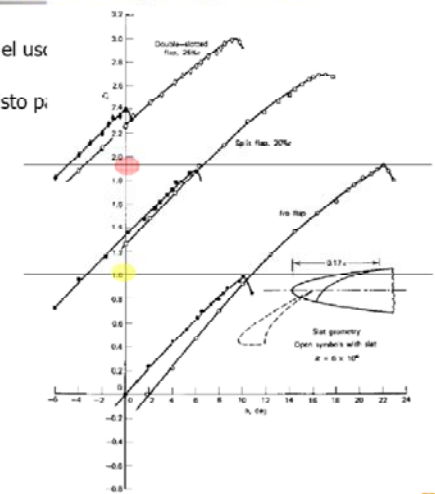
Figure 3.39 Effect of leading edge slat on NACA 64A010 airfoil with and without slat.
