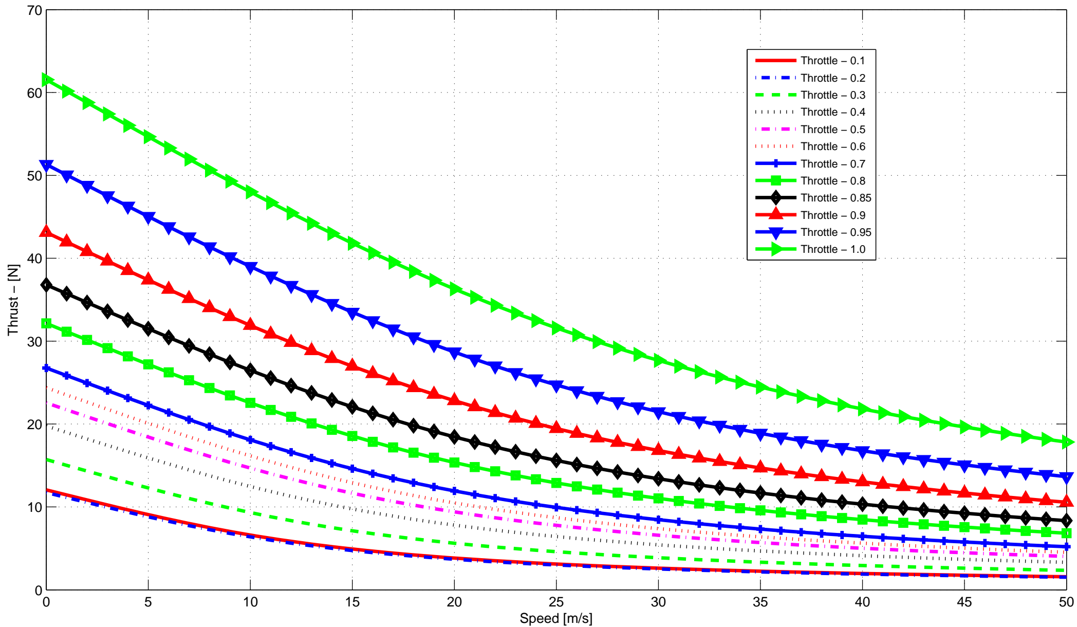
Thrust vs Speed – for variable \delta_T
