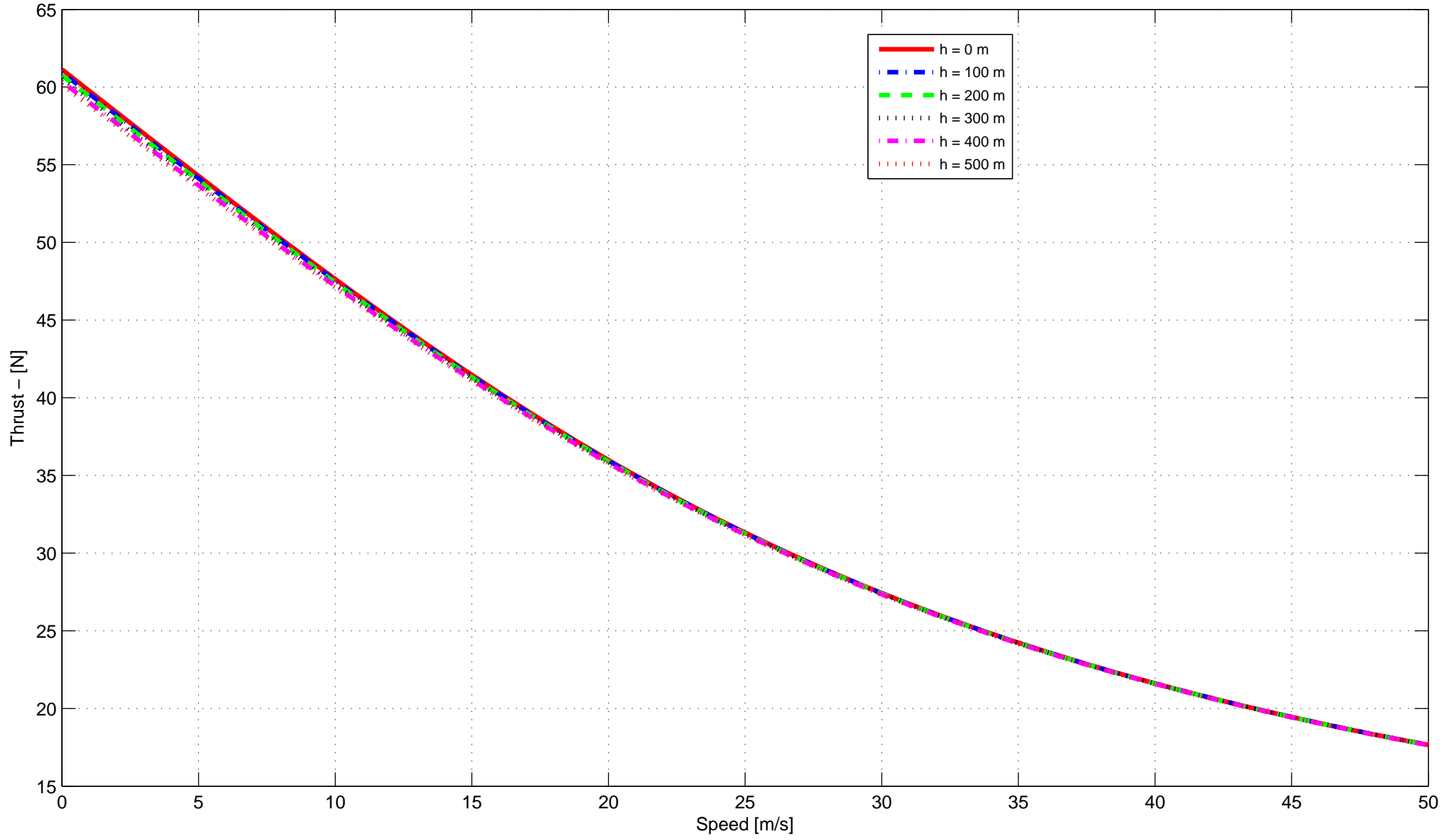
Thrust vs Speed – for variable altitude
