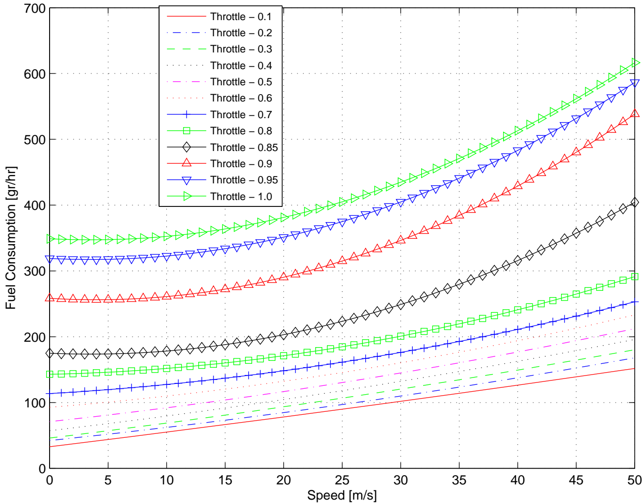
Fuel Consumption vs. Speed for variable \delta_T
