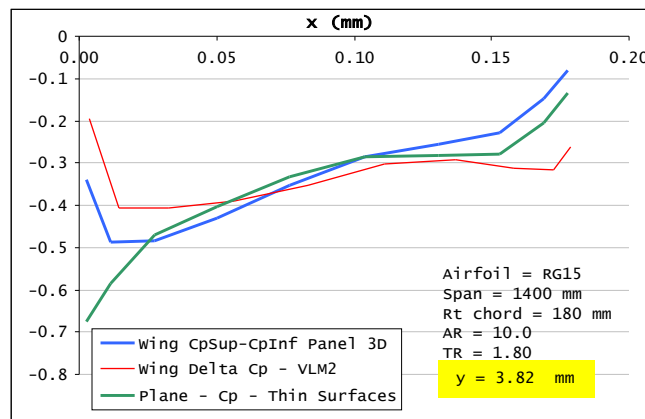
Figure 24 – C_p comparison for different analysis methods
