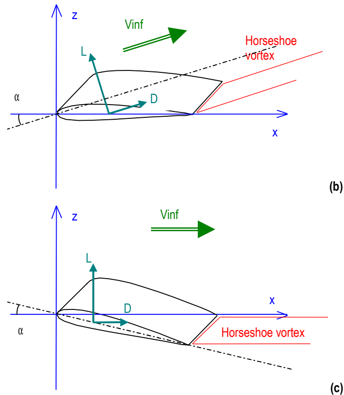
Figure 28 – Normal and Tilted geometry configurations
