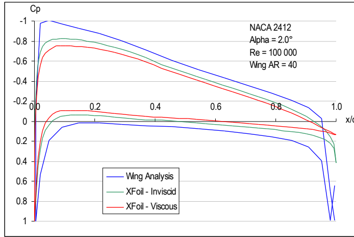
Figure 22 – Pressure Coefficient Analysis – NACA2412
