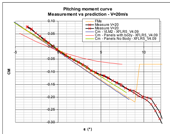
Figure 36 – Predicted pitch moment vs. experimental results
