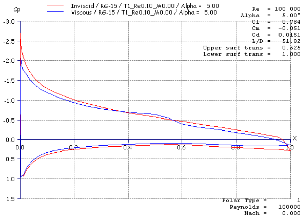
Figure 2 : C_p calculation
