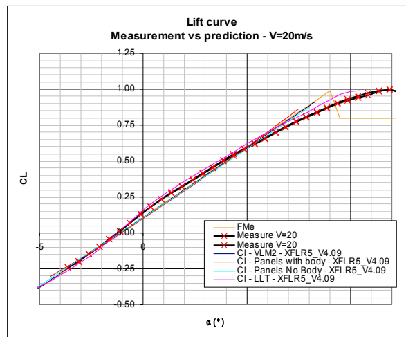
Figure 34 – Predicted lift curve vs. experimental results
