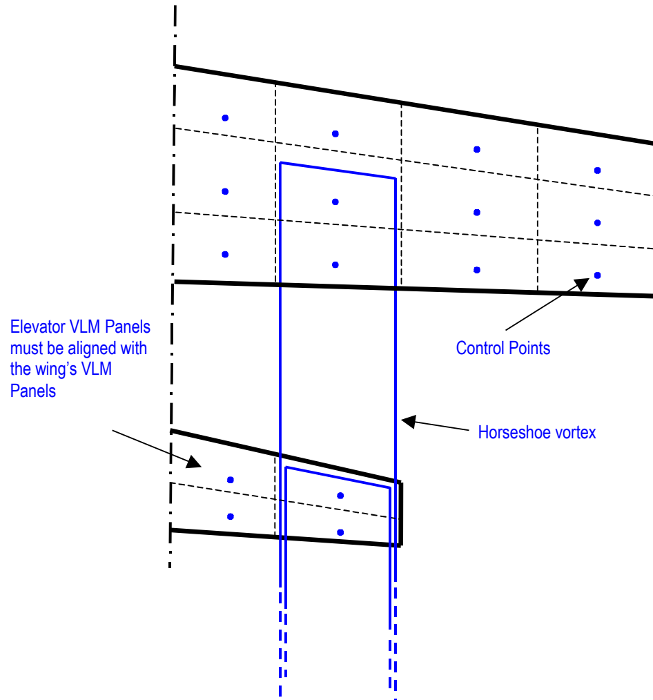
Figure 11: VLM Panel arrangement for a plane
