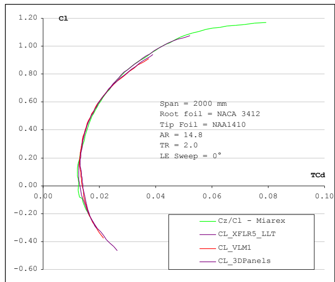
Figure 37 – Comparison to results from Miarex
