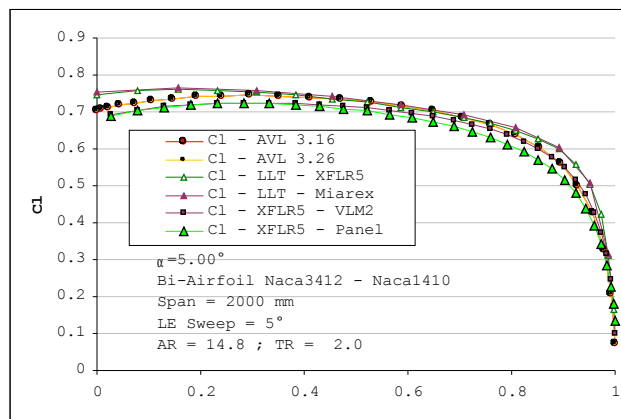
Figure 38 – Lift coefficient - Comparison to AVL and Miarex
