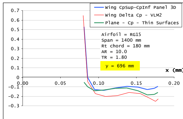
Figure 25 – C_p comparison for different analysis methods
