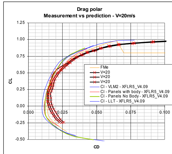
Figure 35 – Predicted drag polar vs. experimental results
