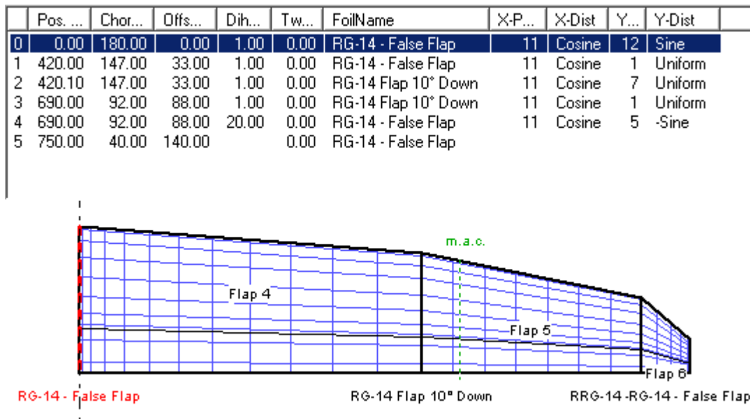
Figure 7 – Flap Definition
