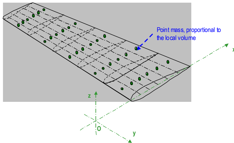
Figure 45 – Mass representation for the wing
