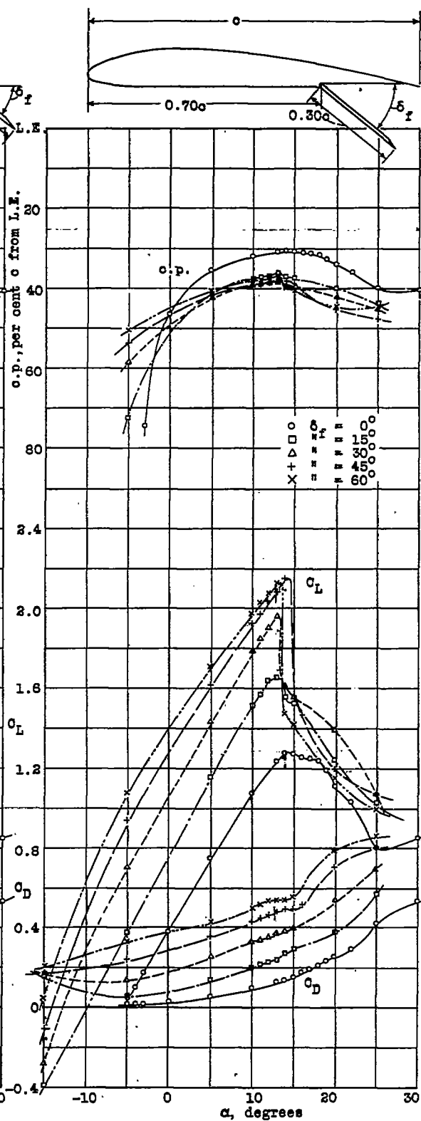
Fig. 5 The 30 per cent c flap hinged at 70 per cent c
