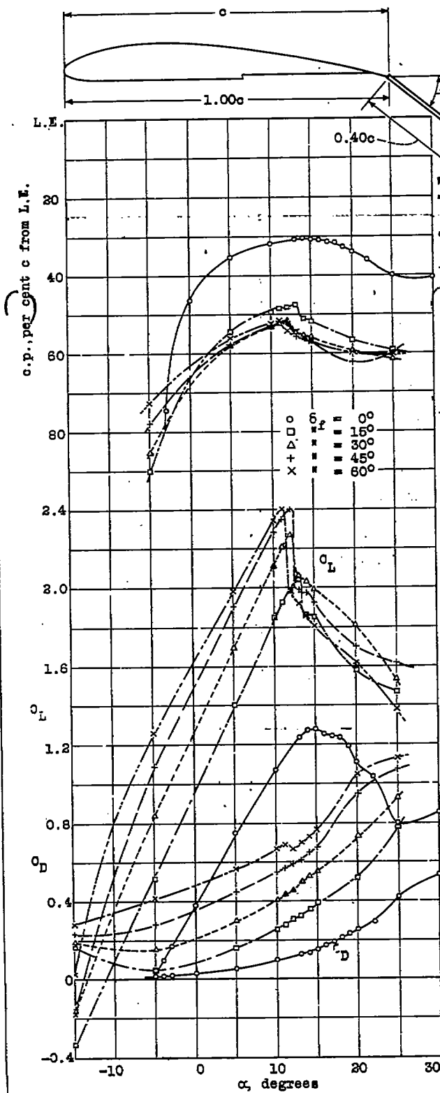
Fig.13 The 40 per cent c flap hinged at 100 per cent c
