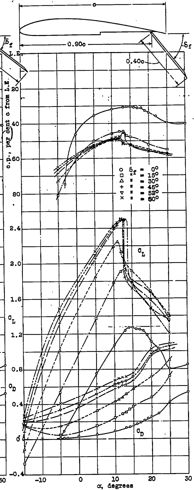
Fig.13 The 40 per cent c flap hinged at 90 per cent c
