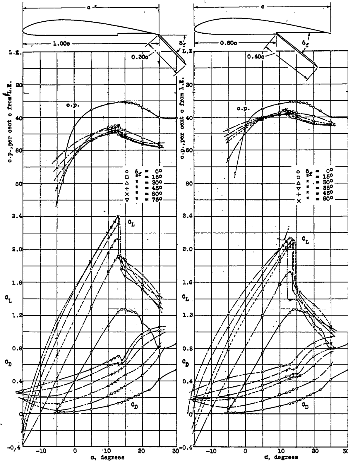
Fig. 8 The 30 per cent c flap hinged at 100 per cent c
