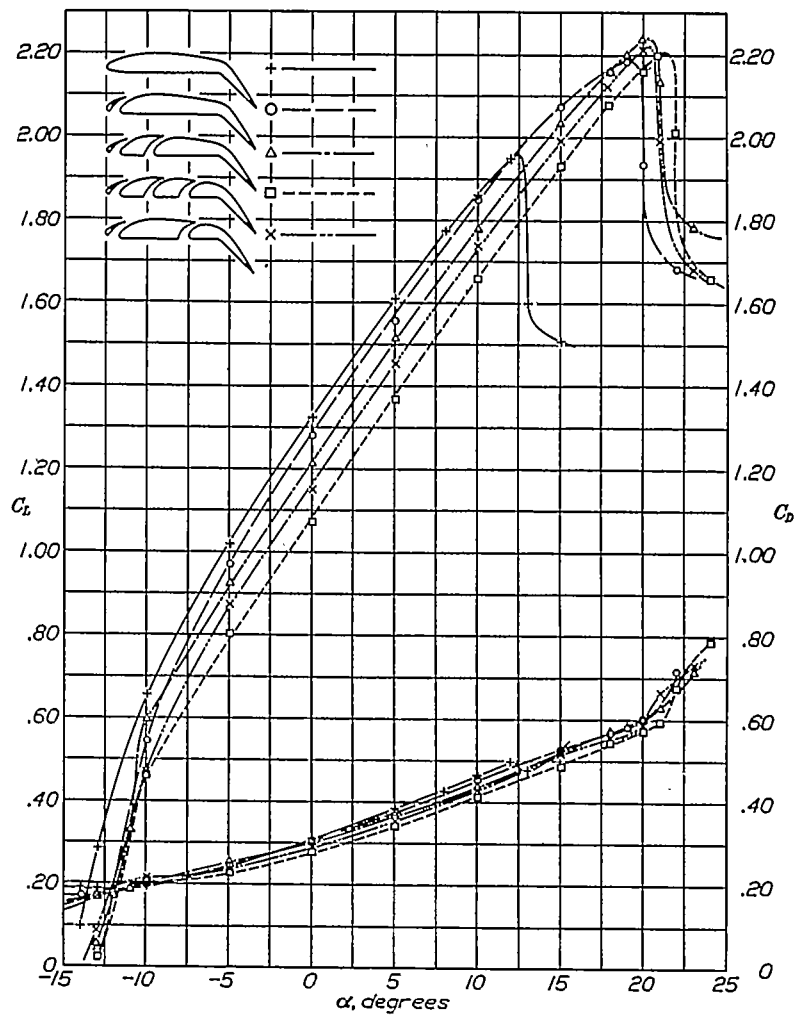
FIGURE 6.—Lift and drag coefficients for a wing with 45° flap and various leading edge and center fixed slots
