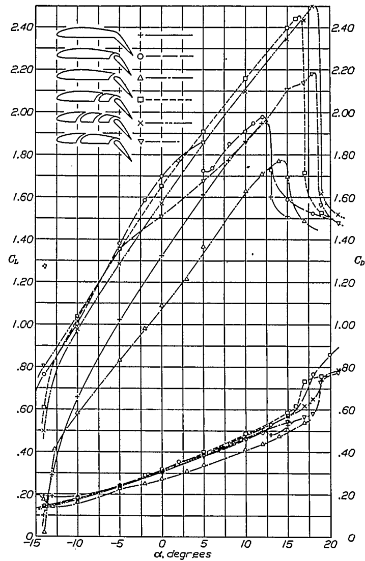
FIGURE 7.—Lift and drag coefficients for a wing with 45° flap and various center and rear fixed slots
