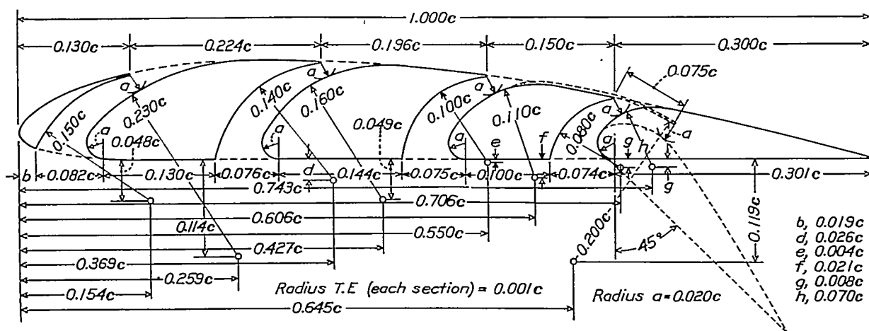
FIGURE 1.—Section of Clark Y wing with multiple fixed slots and trailing-edge flap
