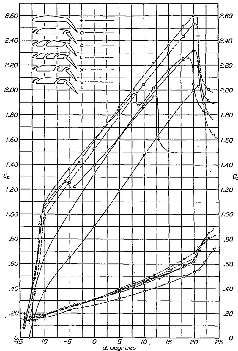
FIGURE 8.—Lift and drag coefficients for a wing with 45° slotted flap and various leading edge and center fixed slots
